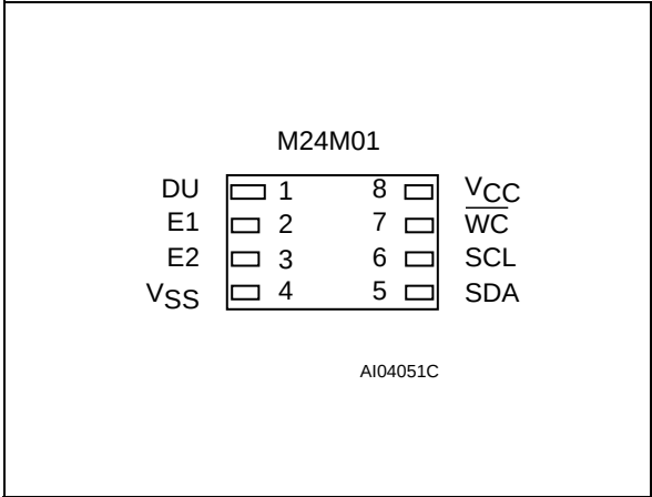
Figure 3. LGA Connections
