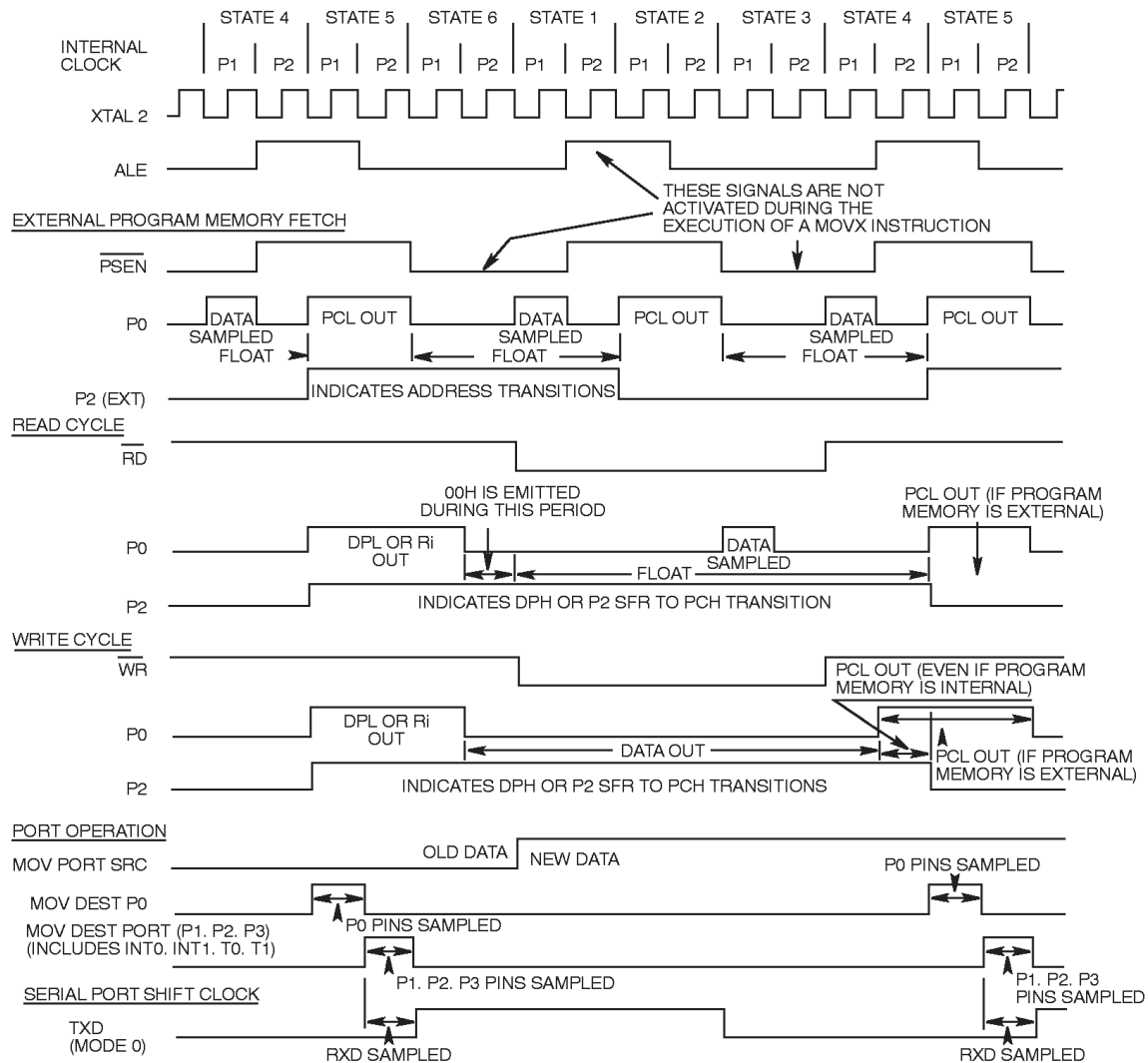
Figure 20. Clock Waveforms
