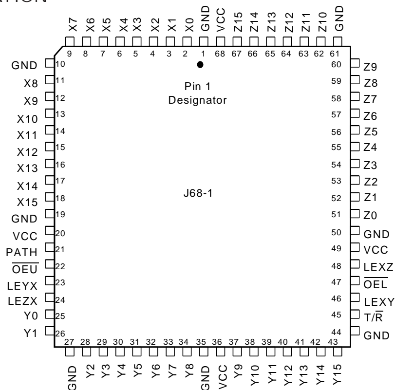
PLCC TOP VIEW
