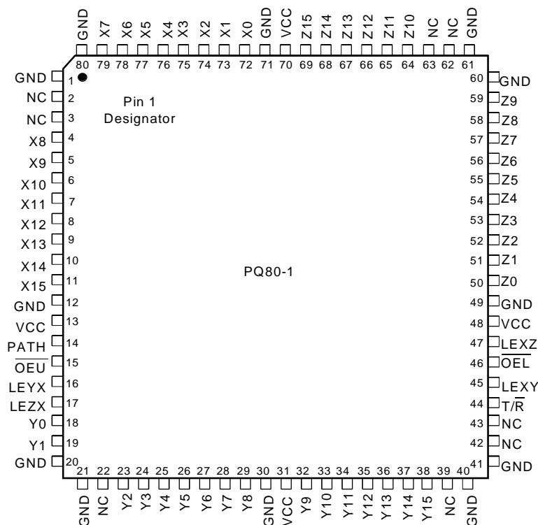
PQFP TOP VIEW
