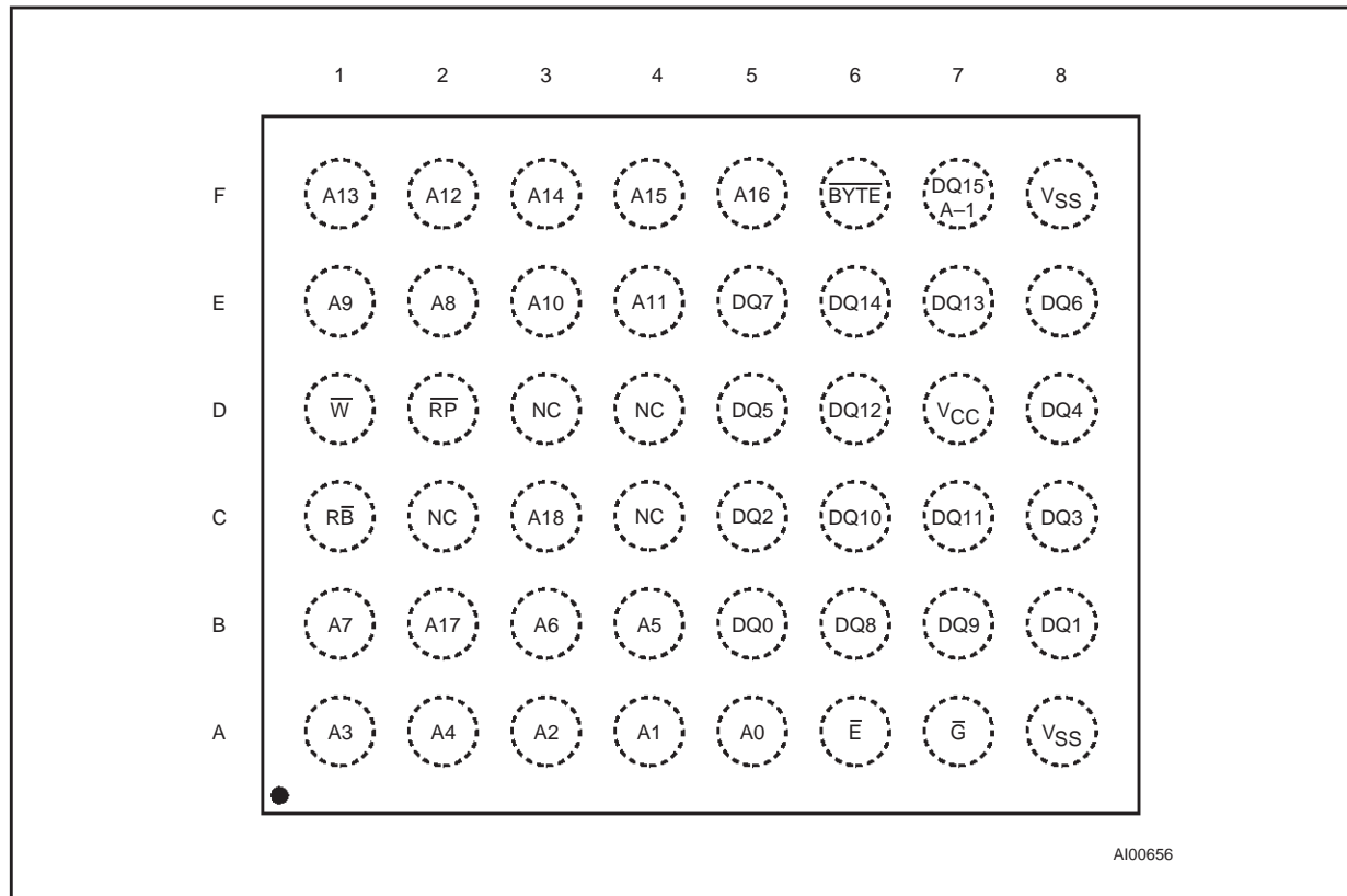
Figure 2C. FBGA Package Ball Out (Top View)
