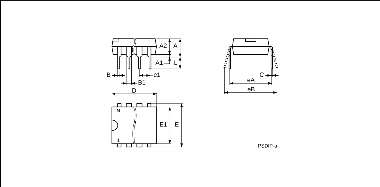
Figure 13. PSDIP8
