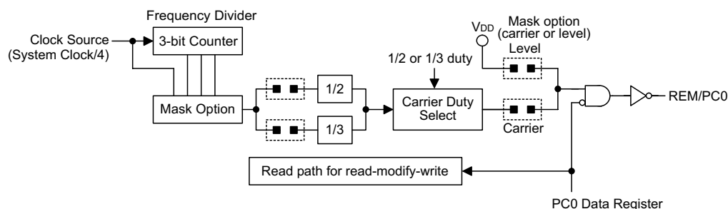
Carrier/Level output
