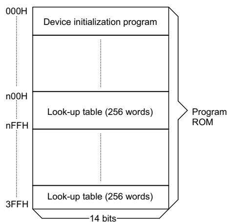
Program memory
