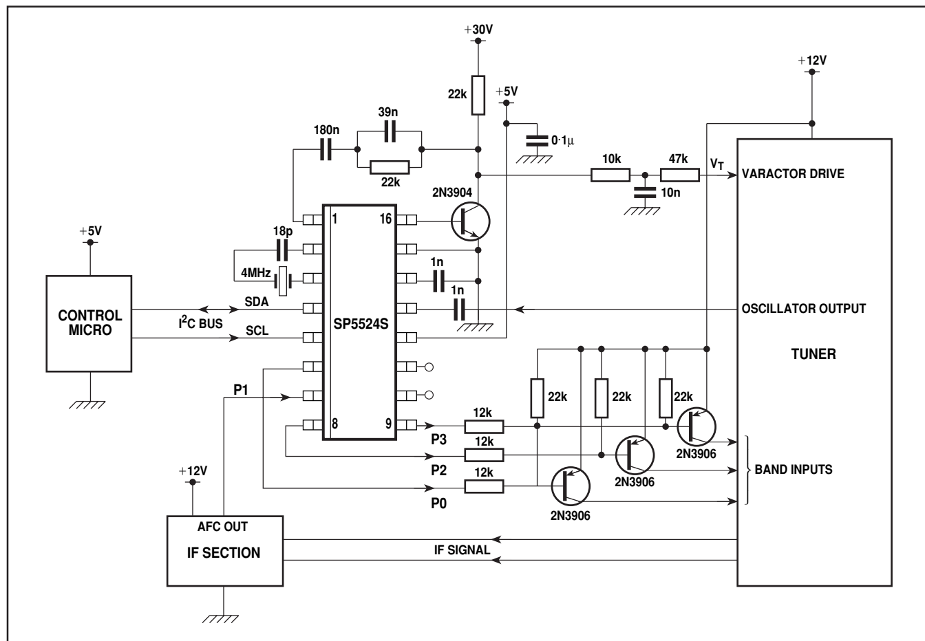
Fig. 4 Typical application
