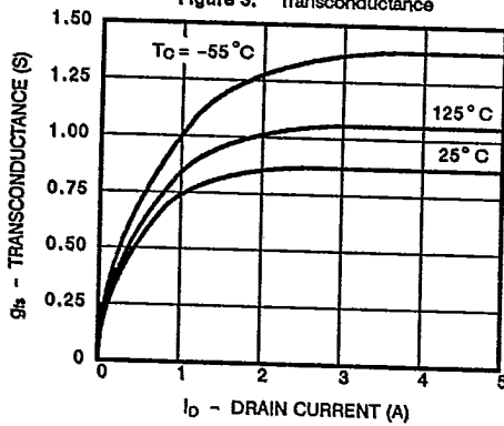
Figure 3. Transconductance
