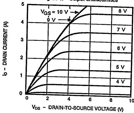
Figure 1. Output Characteristics
