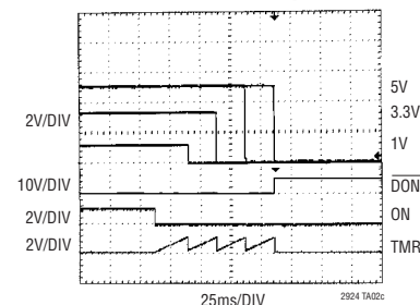
Power-Down Sequence
