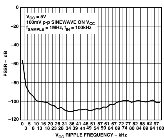
TPC 6. Typical Power Supply Rejection Ratio (PSRR)
