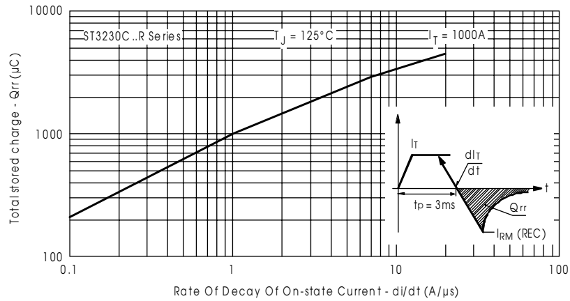
Fig. 7 - Stored Charged
