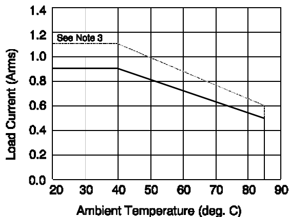
Figure 1. Derating Curve, Free Standing
