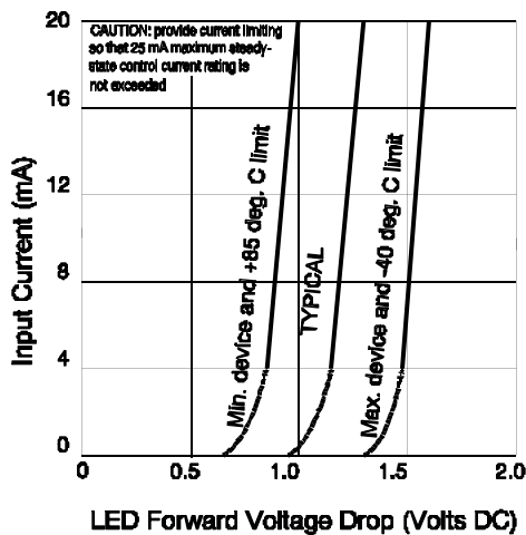
Figure 3. Input Characteristics (Current Controlled)
