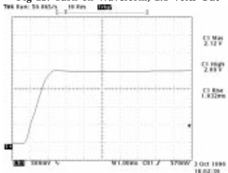
Fig 23. Turn on Waveform, 2.1 Volts Out
