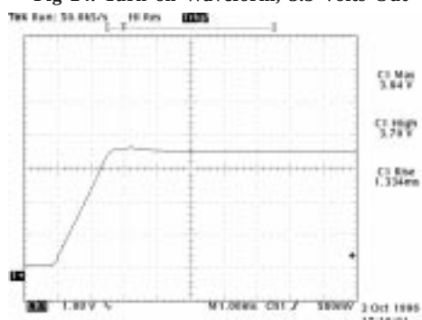
Fig 24. Turn on Waveform, 3.5 Volts Out
