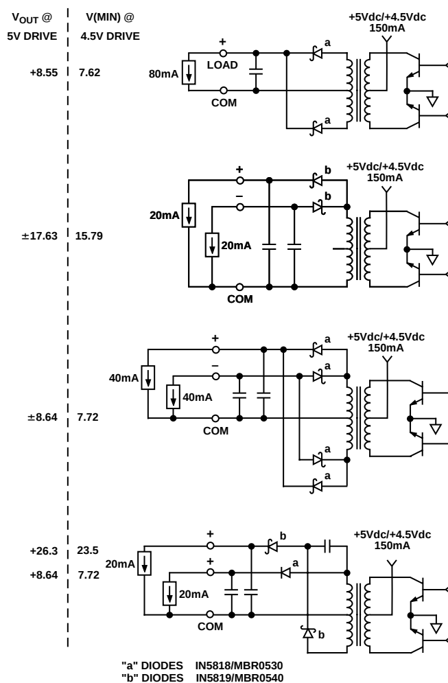
Figure 5. Field Side Power Supply Rectifier Examples
