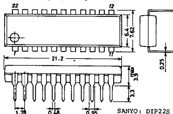
Package Dimensions 3059-D22SIC (unit: mm) [LC7364J]
