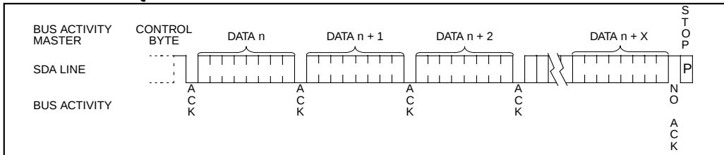
FIGURE 7-3: SEQUENTIAL READ
