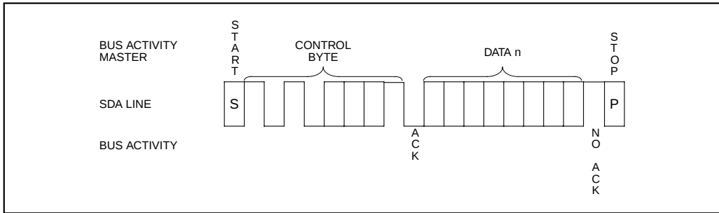
FIGURE 7-2: RANDOM READ
