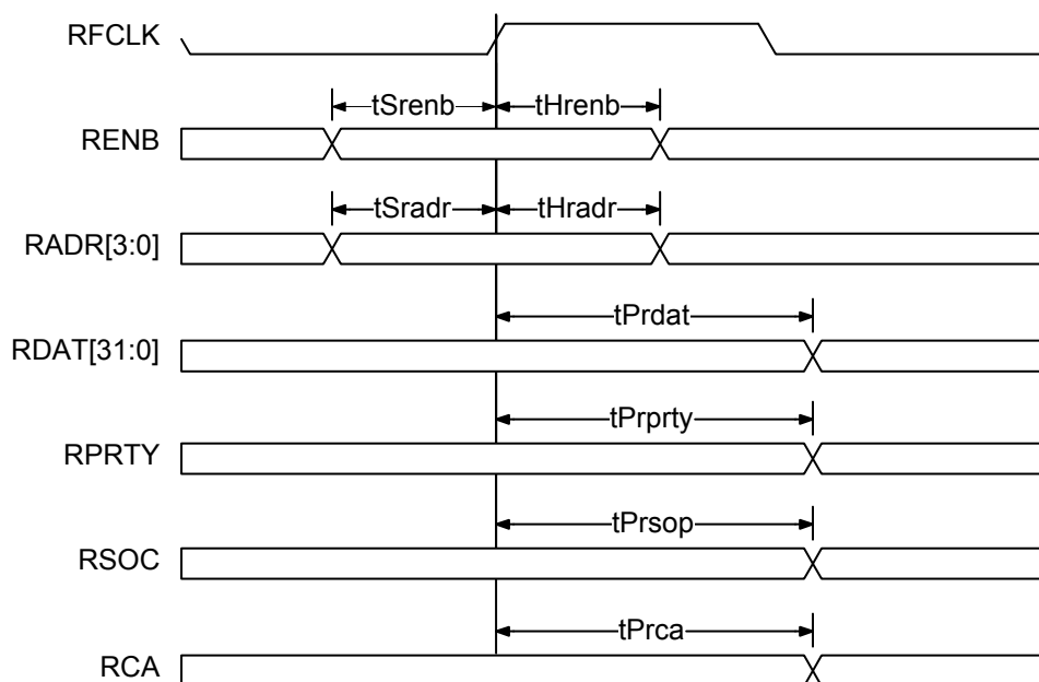
Figure 55: Receive UTOPIA Level 3 System Interface Timing Diagram
