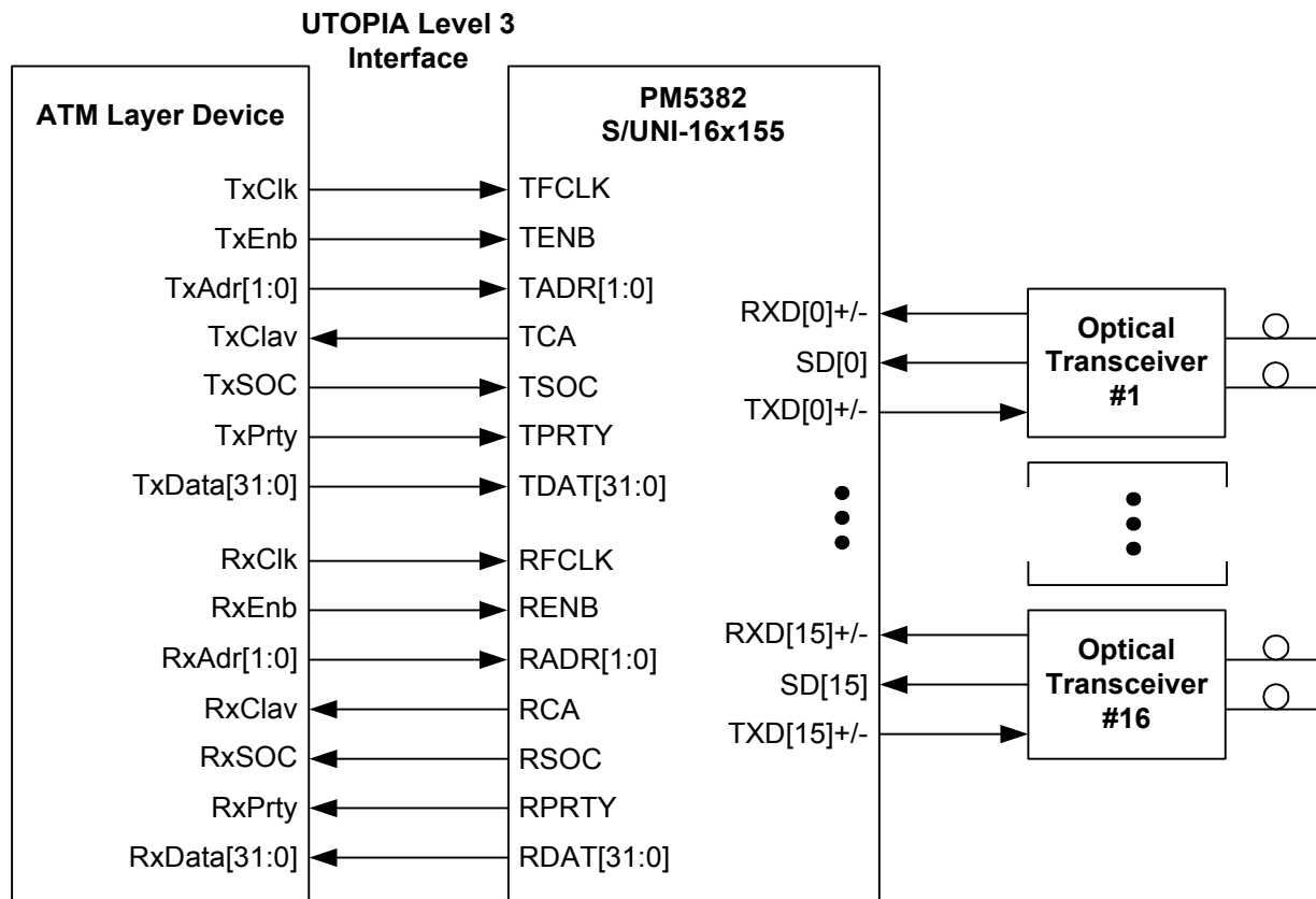
Figure 1: Typical STS-3c/STM-1 ATM Switch Port Application
