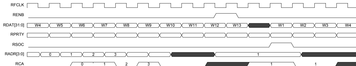
Figure 44: Receive UTOPIA Level 3 System Interface Timing
