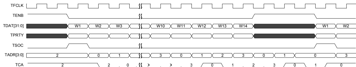
Figure 43: Transmit UTOPIA Level 3 System Interface Timing
