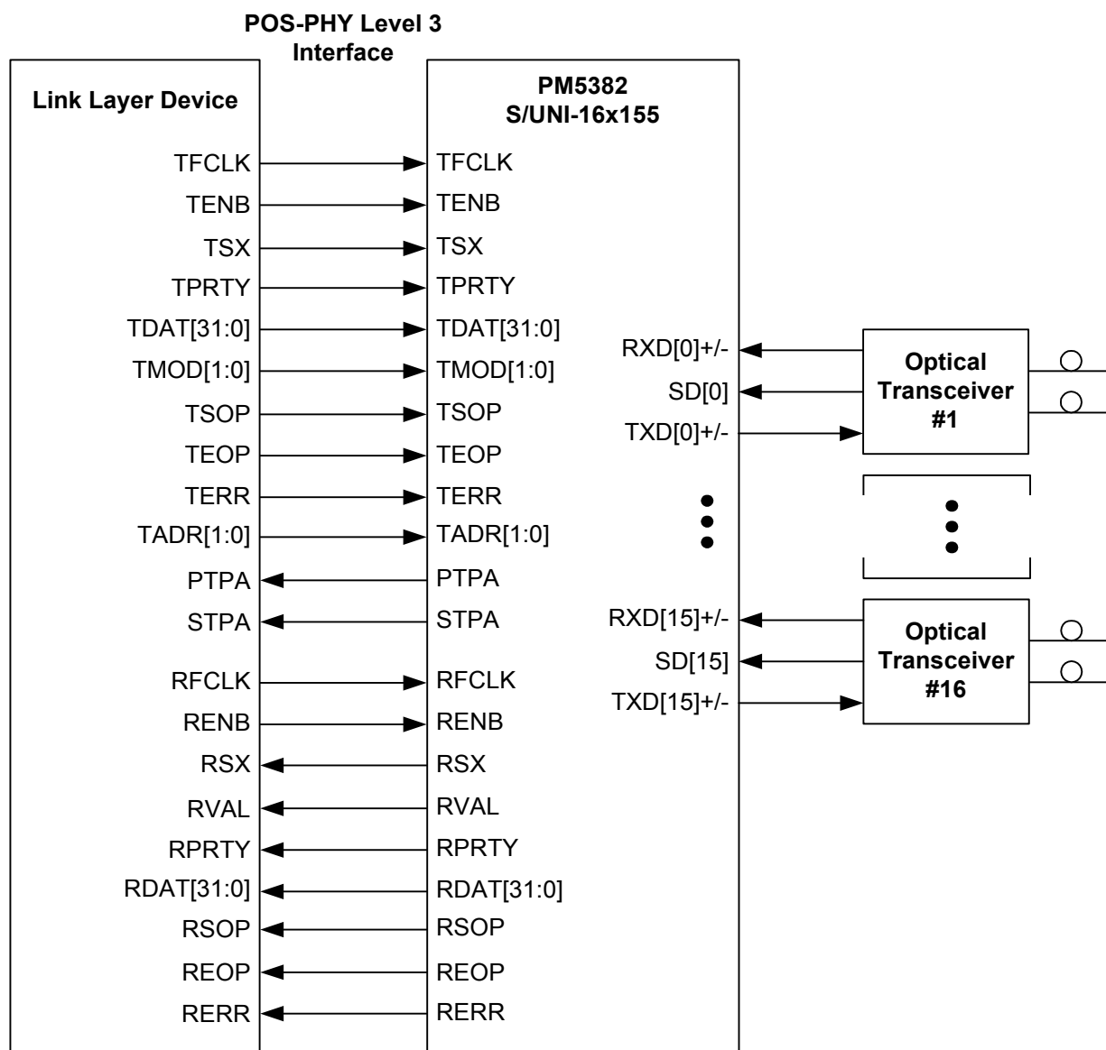
Figure 2: Typical STS-3c/STM-1 Packet over SONET/SDH Application
