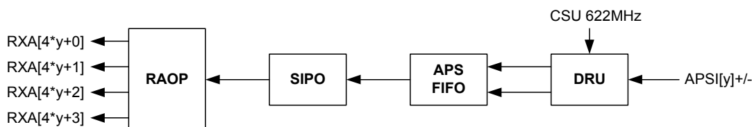
Figure 32: Receive APS Link
