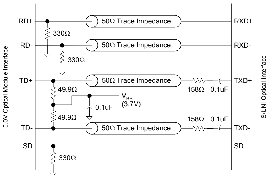
Figure 38: Interfacing S/UNI-16x155 Line PECL Pins to 5.0V Devices
