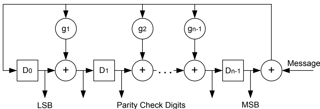
Figure 10: CRC Generator
