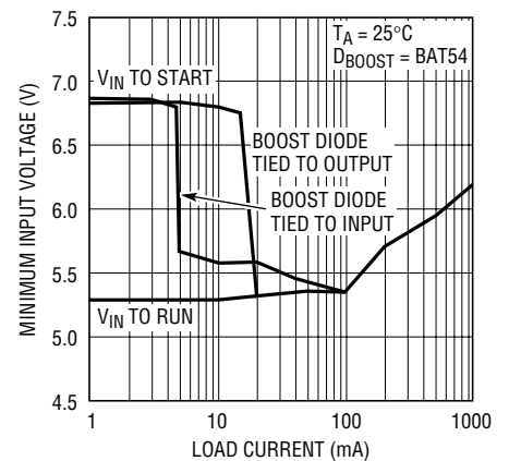
Minimum Input Voltage, V OUT = 5V
