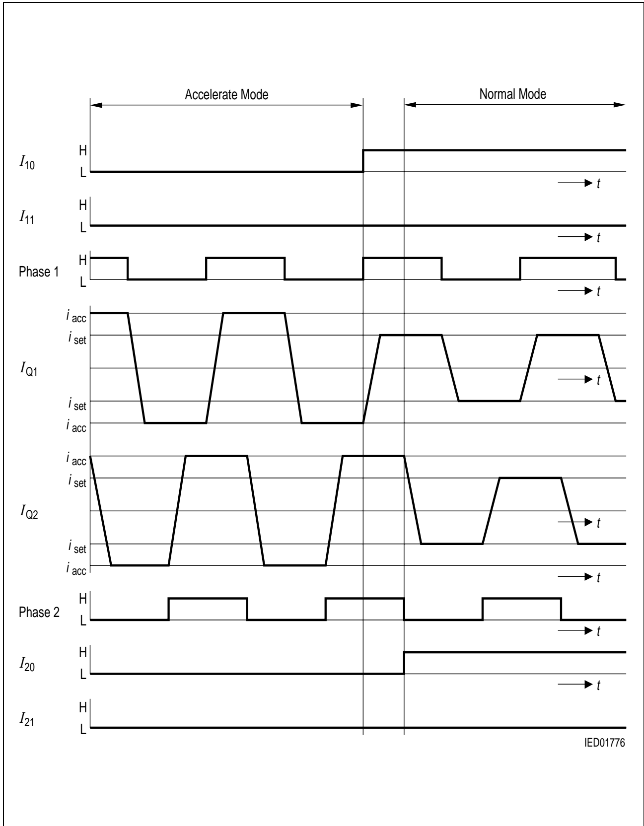
Figure 5 Full-Step Operation
