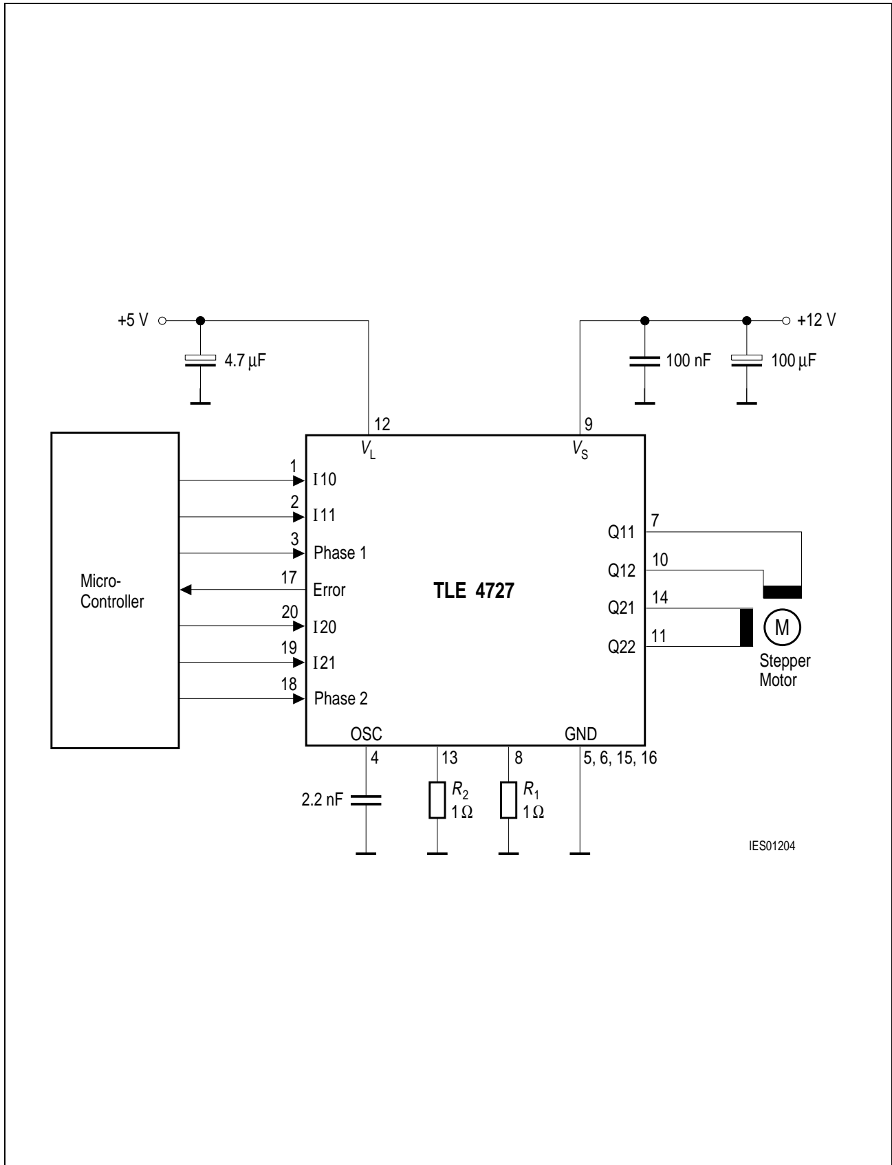
Figure 3 Application Circuit
