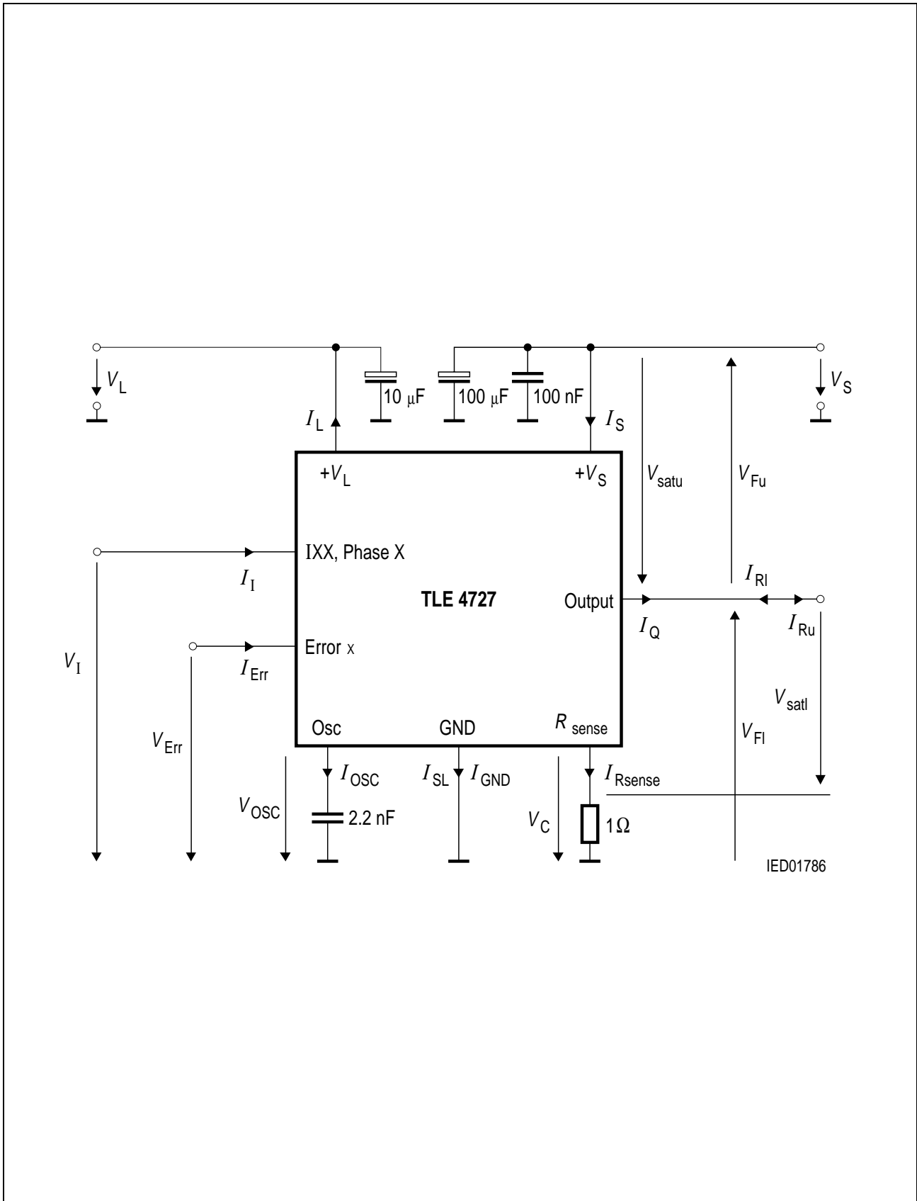
Figure 4 Test Circuit
