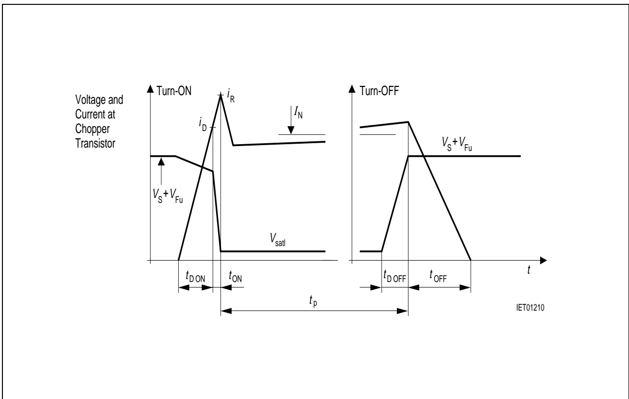
Figure 10 Voltage and Current at Chopper Transistor
