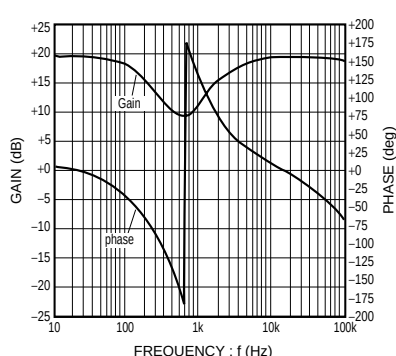
Fig.6 Surround characteristics
