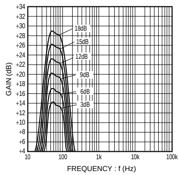
Fig.8 Biamp characteristics (Input common-mode)
