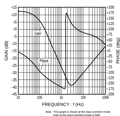
Fig.5 Vocal fade characteristics
