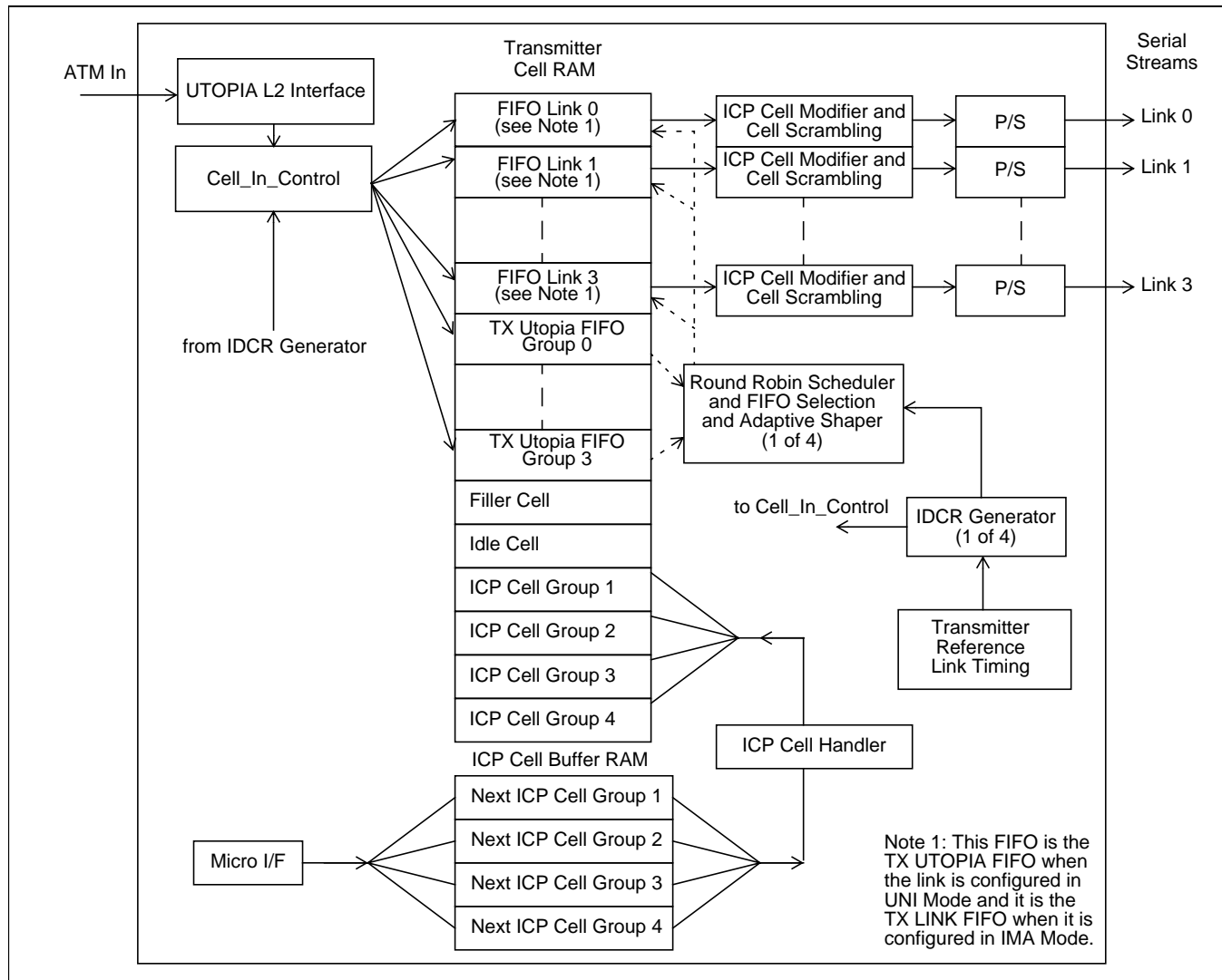
Figure 3 - Functional Block Diagram -Transmitter in IMA Mode
