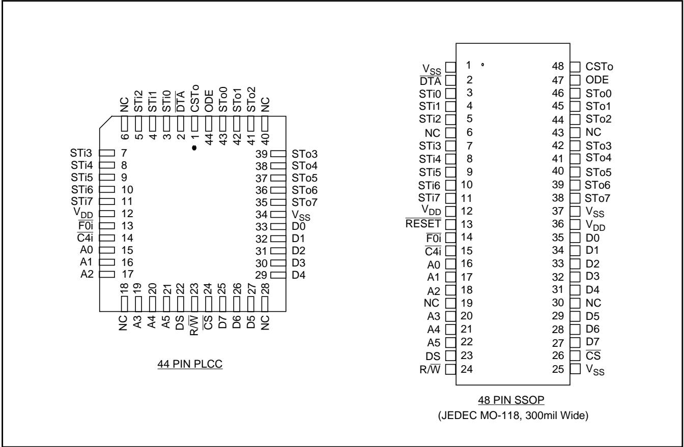
Figure 2 - Pin Connections
