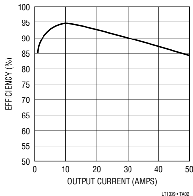
48V to 5V Efficiency Curve
