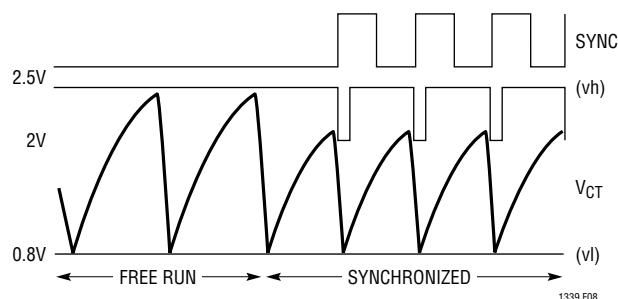
Figure 8. Free Run and Synchronized Oscillator Waveforms (at C_T Pin)
