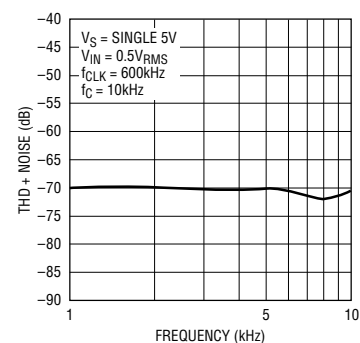
THD + Noise vs Frequency
