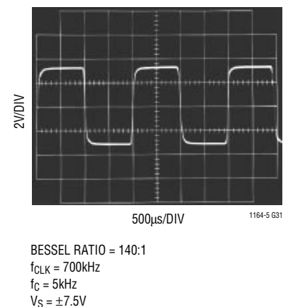
Transient Response V_{IN} = \pm 3\text{V} , 500Hz Square Wave
