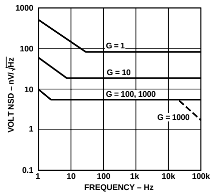
Figure 15. RTI Noise Spectral Density vs. Gain
