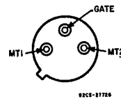
Modified TO-205
