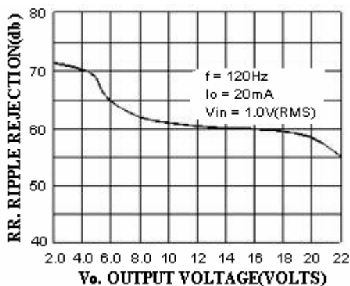
FIGURE 5 - RIPPLE REJECTION AS A FUNCTION OF OUTPUT VOLTAGES
