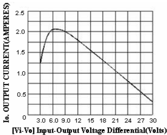
FIGURE 3 - PEAK OUTPUT CURRENT AS A FUNCTION OF INPUT-OUTPUT DIFFERENTIAL VOLTAGE
