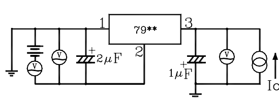
TEST CIRCUIT 2
