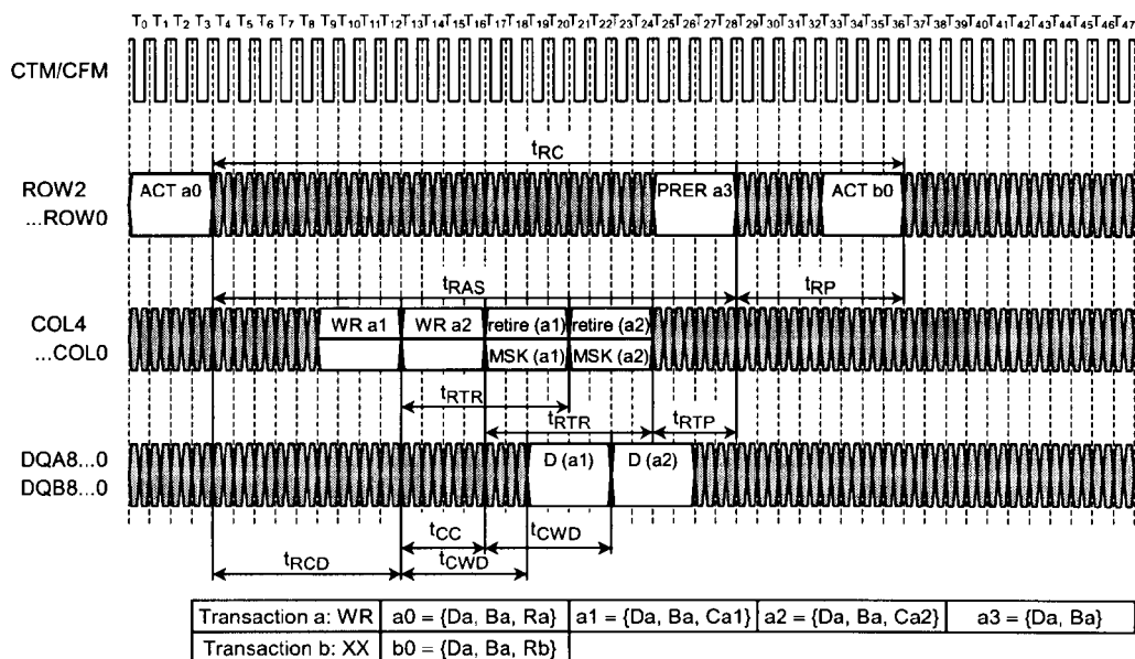
Figure 17. Write Transaction Example
