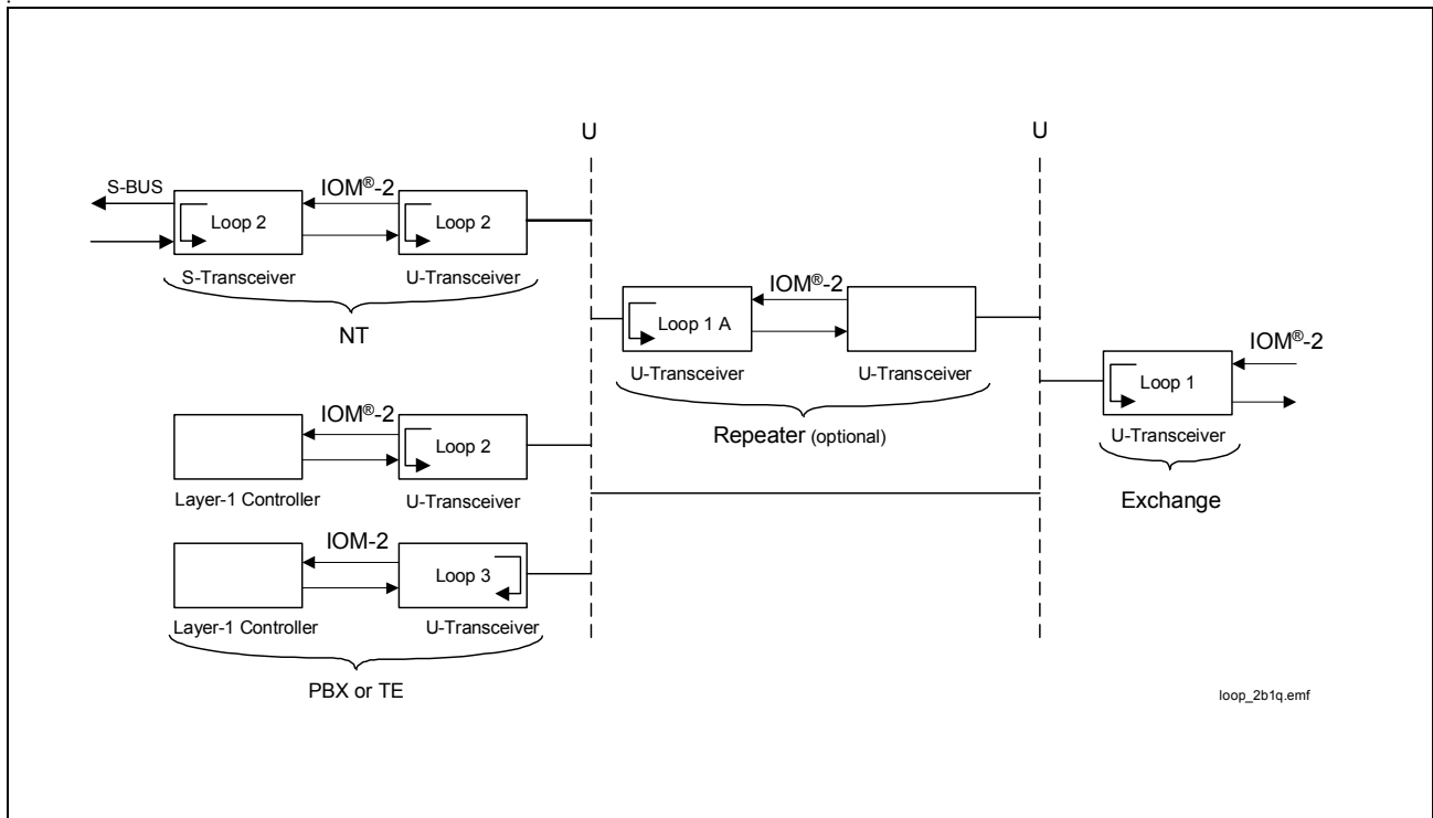
Figure 49 Test Loopbacks
