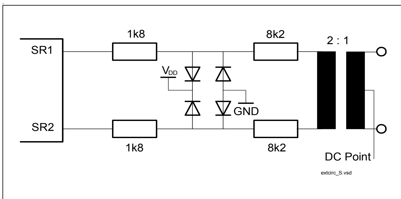
Figure 56 External Circuitry S-Interface Receiver
