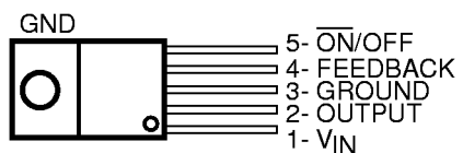
5-LEAD TO-220 (T)
