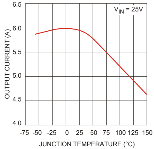
Figure 3. Current Limit
