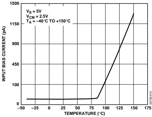
Figure 14. AD8628 Input Bias Current vs. Temperature
