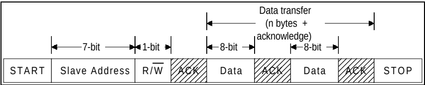
Figure 7-24. Bus Protocol
