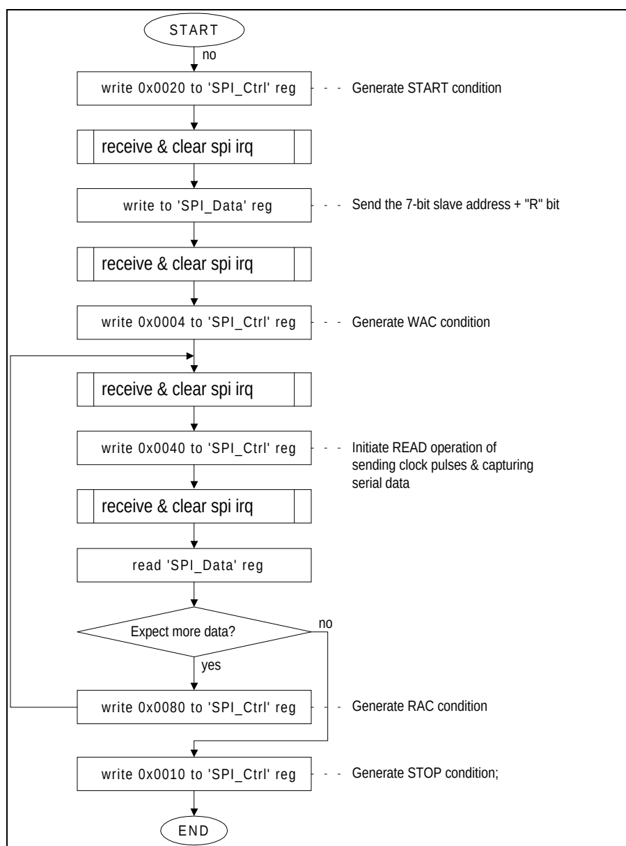
Figure 7-28. Firmware Operation—Reception
