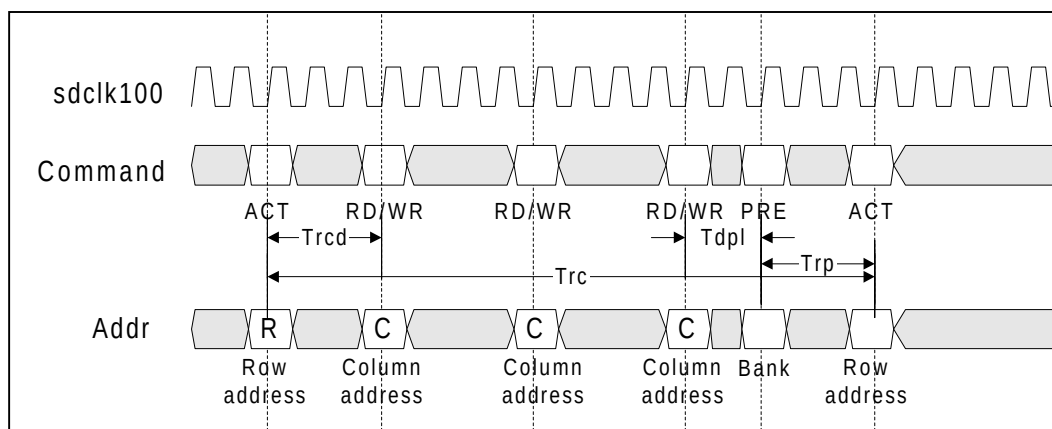
Figure 24-3. SDRAM Read or Write Timing
