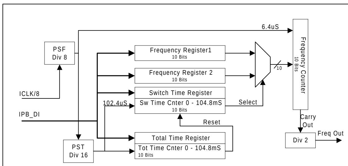
Figure 20-5. Dual-Tone Tone Generator Block Diagram
