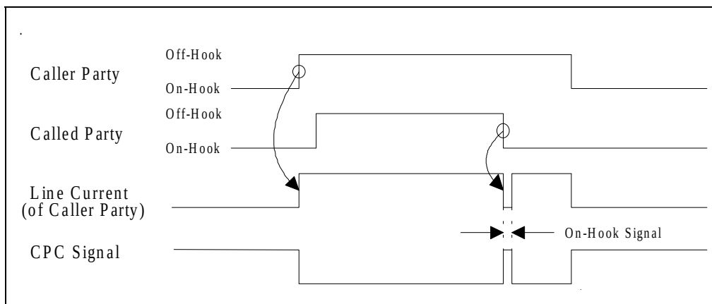
Figure 22-1: CPC Signal
