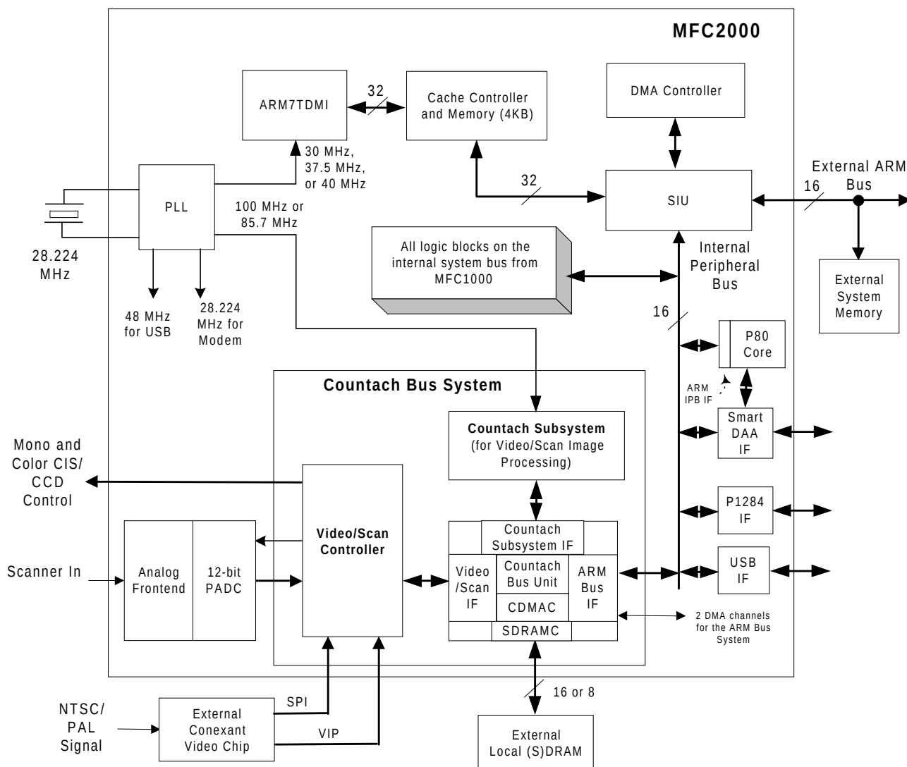
Figure 1-2: MFC2000 Function Diagram
