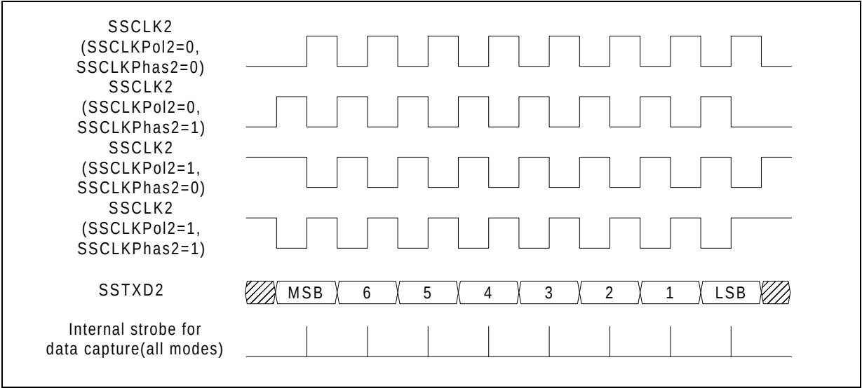
Figure 19-3. SSCLK2 Diagram
