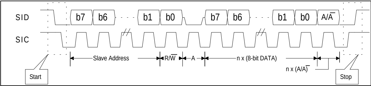
Figure 7-24. Bus Protocol
