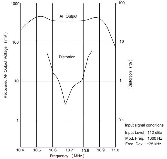
Frequency Characteristics
