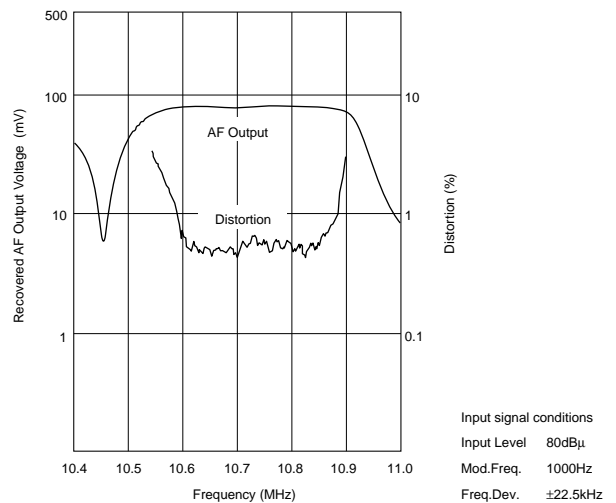
Frequency Characteristics
