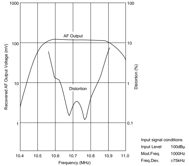
Frequency Characteristics
