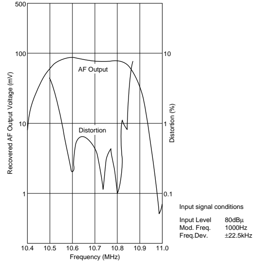
Frequency Characteristics
