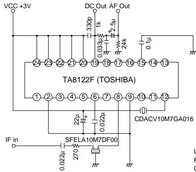
Test Circuit
