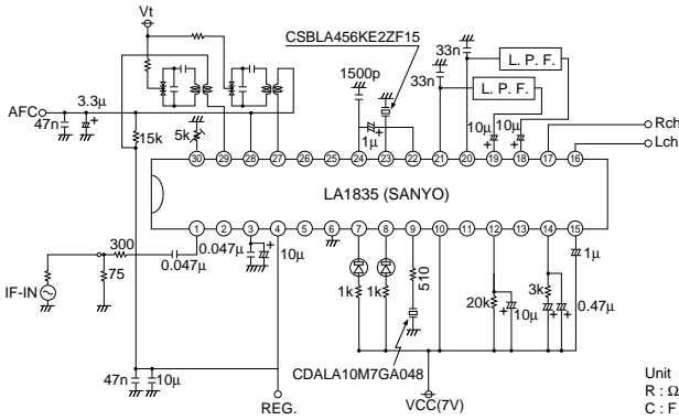
Test Circuit
