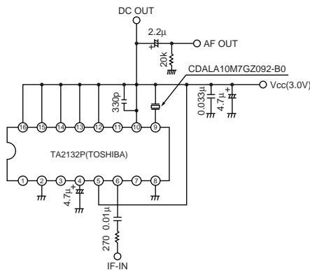
Test Circuit
