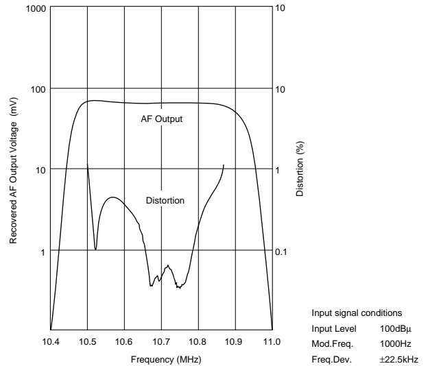
Frequency Characteristics
