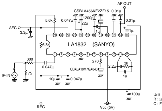
Test Circuit
