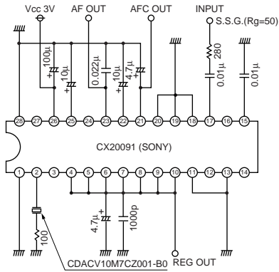
Test Circuit
