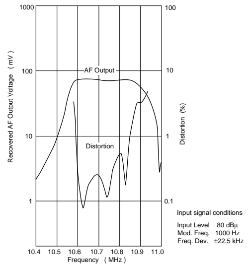
Frequency Characteristics
