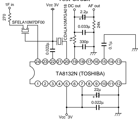
Test Circuit
