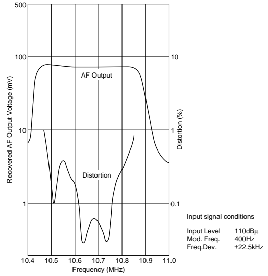
Frequency Characteristics
