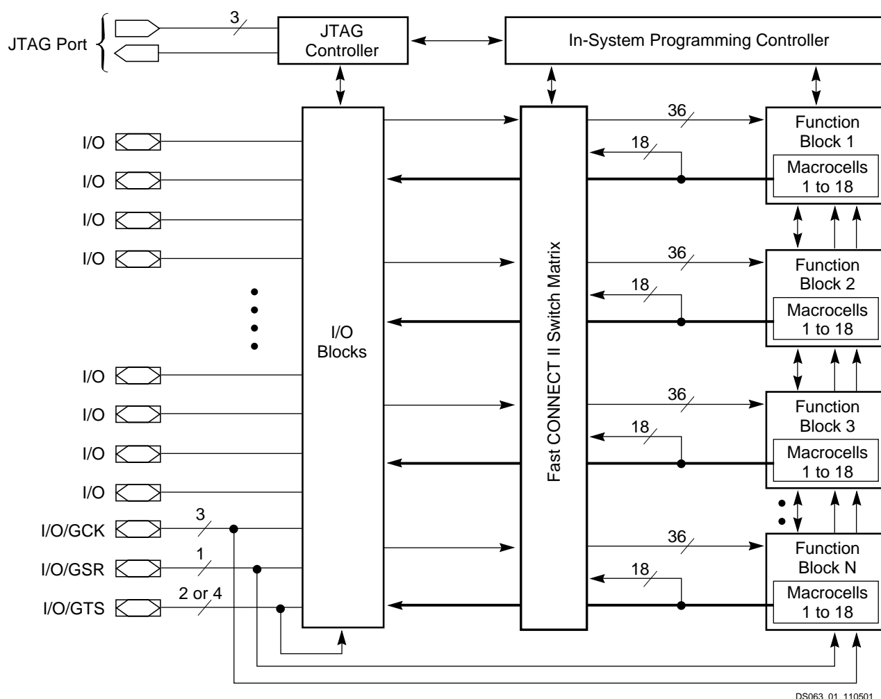
Figure 1: XC9500 Architecture
