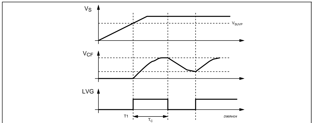
Figure 2. Waveforms
