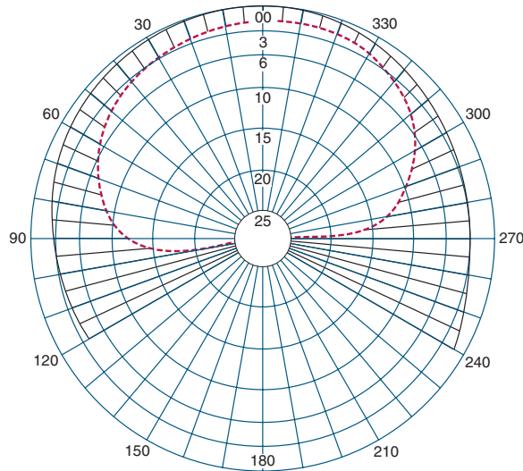
Axial Ratio vs. Elevation Angle
