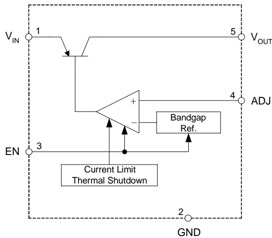
Adjustable Regulator
