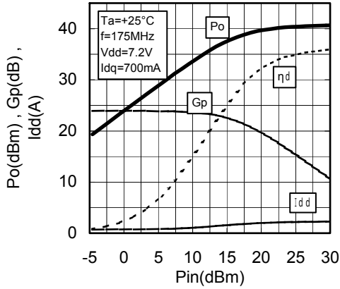
Pin-Po CHARACTERISTICS @f=175MHz
