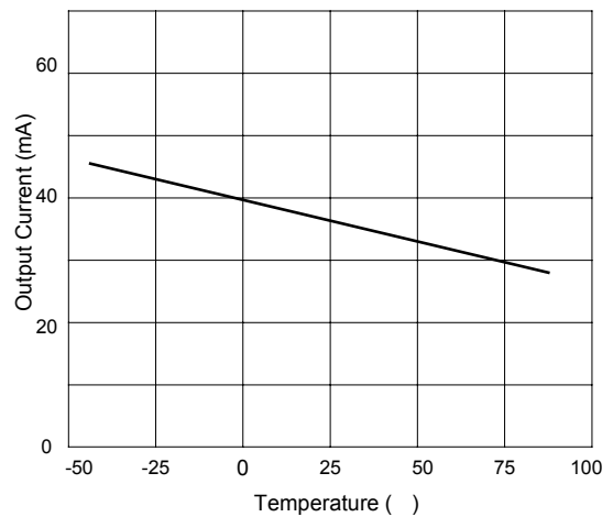
Fig.11 Current Limiting
