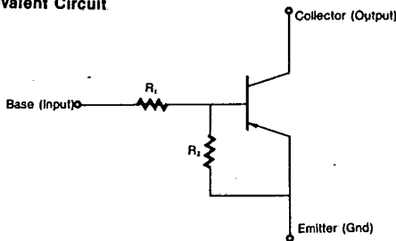
Equivalent Circuit
