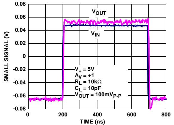
FIGURE 14. SMALL SIGNAL STEP RESPONSE RISE AND FALL TIME
