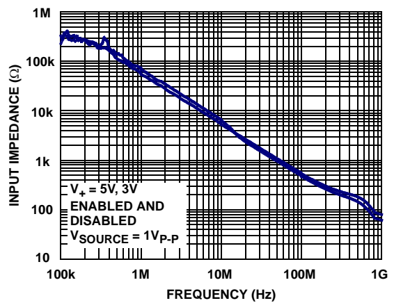
FIGURE 4. INPUT IMPEDANCE vs FREQUENCY
