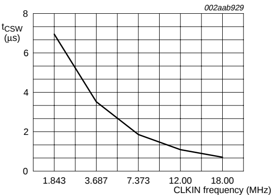
Fig 24. t CSW as a function of CLKIN frequency
