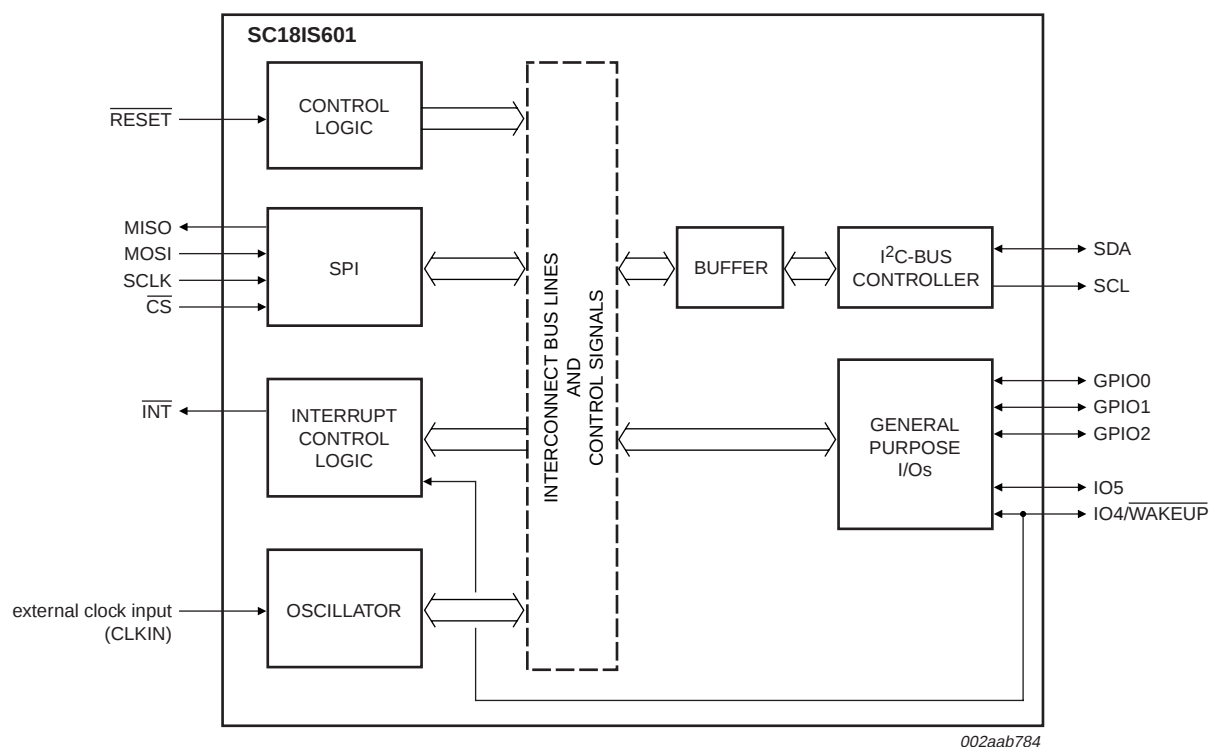
Fig 2. Block diagram of SC18IS601
