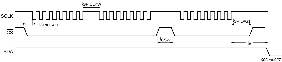
Fig 23. SPI to I 2 C-bus timing diagram
