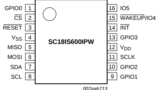
Fig 3. SC18IS600 pin configuration for TSSOP16
