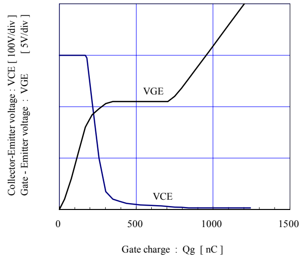
Dynamic Gate charge (typ.) V_{CC} = 300\text{V} , I_C = 300\text{A} , T_j = 25^\circ\text{C}
