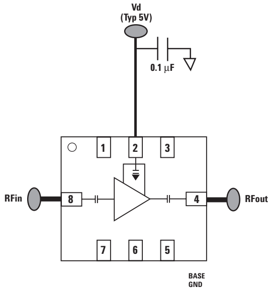
Figure 19. Typical Application.
