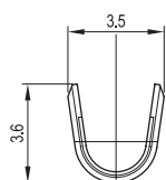
SECTION B-B'
