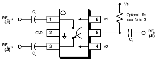
Figure 1: Pin Layout
