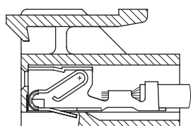
TERMINAL ASSEMBLY DRAWING
