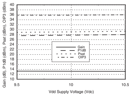
Gain, Power & OIP3 vs. Supply Voltage @ 10 GHz, Fixed Vgg
