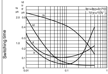
Switching Speeds
